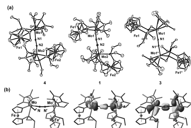
Figure 1. Molecular structures of dinitrogen-bridged dimolybdenum complexes. a) Crystallographic structures of the main parts of 4 , 1 , and 3 . b) Optimized structure of 3 in the triplet spin state and spatial distribution of the SOMOs (HOMO-1 (left) and HOMO (right)).
